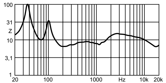
Impedanzgang Q-10 impedance Q-10
